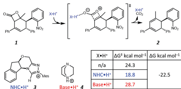
Fig. 1 Illustration of the NHC- H^+ catalysed decarboxylation of 1 proposed by Zhang et al. 14 The Gibbs free energy barriers and reaction free energies were calculated at B3LYP-D3/6-311++G(2df,2pd)/SMD(NMP/tBuOH)//B3LYP-D3/6-31G(d,p)/SMD(NMP/tBuOH).
