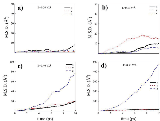
Fig. 9 Cartesian components of the mean squared displacement (MSD) of the hydrogen atoms belonging to water molecules composing the methane–water mixture at field strengths equal to 0.20 V Å −1 (a), 0.30 V Å −1 (b), 0.40 V Å −1 (c), and 0.50 V Å −1 (d).
