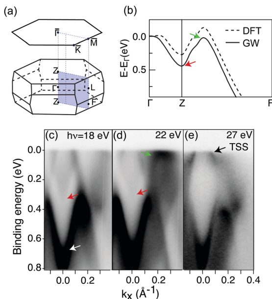
Fig. 1 (a) Bulk Brillouin zone of Sb 2 Te 3 together with the projected surface Brillouin zone. The VB maximum is predicted to be placed either near \bar{\Gamma} or in the shaded plane along the \bar{\Gamma} - \bar{M} azimuthal direction. (b) Calculations of the bulk band structure using density functional theory with and without additional GW corrections from ref. 10 and 11, respectively. The calculations have been shifted so as to align at the band maximum at \bar{\Gamma} , E_F , which is also chosen as the energy zero. (c)–(e) Photoemission intensity as a function of binding energy and k_x (in the direction along \bar{\Gamma} - \bar{M} ), collected at photon energies of 18, 22 and 27 eV, respectively. Several features are marked: the bottom of the VB along \bar{\Gamma} - \bar{Z} (red arrow), the branch of the VB forming a local maximum in the shaded plane (green arrow), the topological surface state (TSS, black arrow) and a further deeper lying surface state (white arrow). The photoemission intensity is scaled such that dark corresponds to high intensity and the colour scale has been saturated to show the relevant features at the Fermi level.
