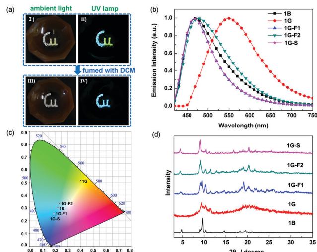
Fig. 3 (a) Photos of various states of 1B during the ground-fumed conversion. Photos I and III were taken under ambient light, while photos II and IV were taken under a UV lamp (365 nm). In photos I and II, the letters "C" and "u" are made up of 1B and 1G samples, respectively. Photos III and IV show the state after fumigation with DCM, where the luminescent color of the letter "u" changed from yellow to blue. (b) Photoluminescence spectra of various states of 1B during the ground-fumed/soaking conversion. (c) The CIE 1931 chromaticity diagram of various states of 1B during the ground-fumed/soaked conversion. It should be noted that the coordinate points of 1G-F1 and 1G-S are almost coincident. (d) Powder X-ray diffraction (PXRD) spectra of the various states of 1B during the ground-fumed/soaked conversion.
