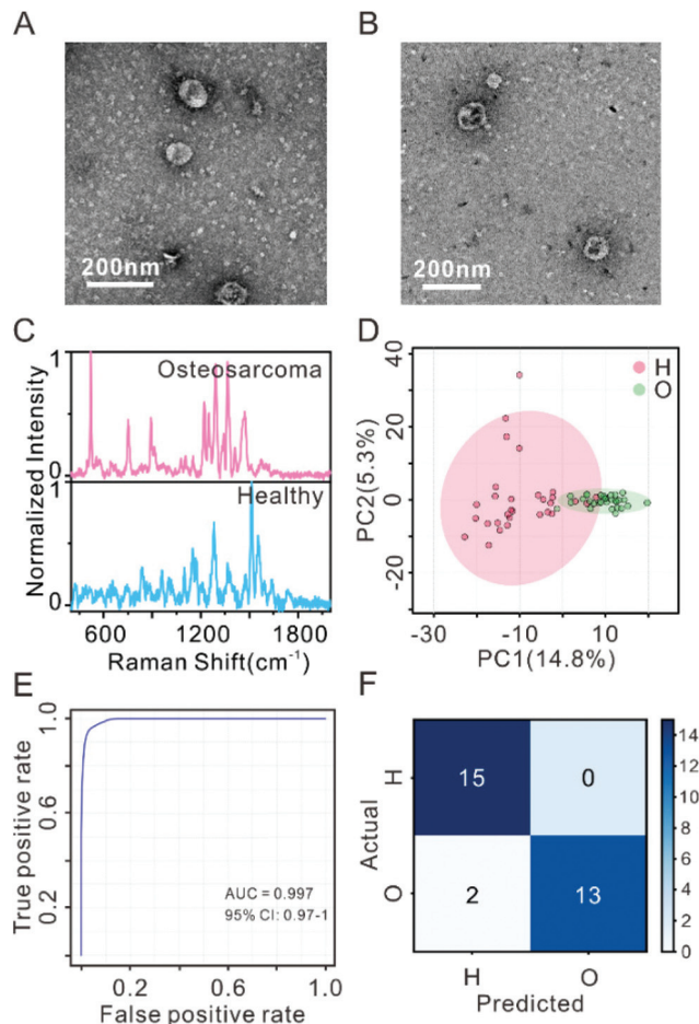
Fig. 3 TEM micrographs of exosomes derived from (A) an osteosarcoma patient and (B) a healthy control. (C) SERS signals of plasma-derived exosomes in the range of 530\text{--}2000\text{ cm}^{-1} from an osteosarcoma patient and a healthy control. (D) PCA score plot of SERS data of plasma-derived exosomes from 10 healthy controls (H) and 10 osteosarcoma patients (O) in the training dataset, with three replicates for each sample. (E) ROC analysis with cross-validation on the training data using classification models built by PLS-DA. (F) Confusion matrix of the classification results of another 5 healthy controls (H) and 5 osteosarcoma patients (O) with three replicates for each sample. The classification model was built by PLS-DA using all the training data.
