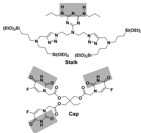
Fig. 1 Structures of Stalk precursor and Cap .
