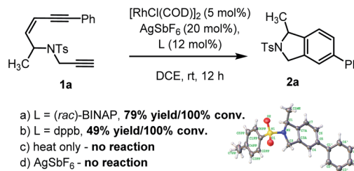
Scheme 2 Initial cycloaromatisation reaction discovery using: (a) L = ( rac )-BINAP; (b) L = dpbb; (c) heat only; or (d) AgSbF 6 alone.
