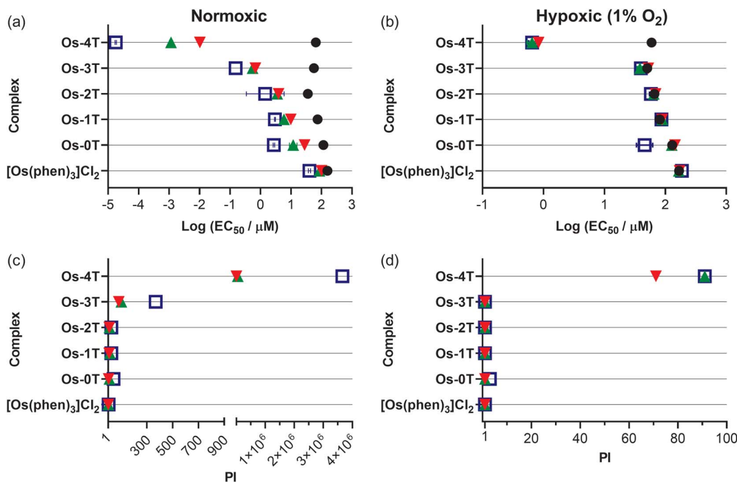
Fig. 9 Summary resazurin-based (photo)cytotoxicity of Os-0T–Os-4T compared to reference compound [\text{Os}(\text{phen})_3]\text{Cl}_2 against SK-MEL-28 in normoxia (18.5–21% \text{O}_2 ; 106 left-column (a and c)) and hypoxia (1% \text{O}_2 ; right-column (b and d)). The phototherapeutic index (PI) as the ratio of light to dark cytotoxicity is plotted in (c) and (d). Figures are labelled as dark (no light; black circles) and 100 \text{ J cm}^{-2} treatments at \sim 20 \text{ mW cm}^{-2} as cool white visible (blue, open square), 523 nm (green, triangle) and 633 nm (red, inverted triangle). Results are tabulated in Tables S-4–S-7.†
