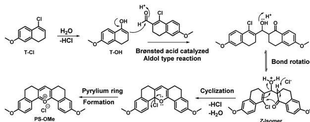
Fig. 1 Possible mechanism of formation of PS-OMe .
