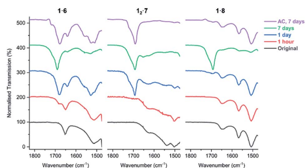
Fig. 11 The FTIR spectra of salts 1 · 6 , 1 2 · 7 , and 1 · 8 in the range of 1475–1825 cm -1 showing the carboxylate environment of the salts with volatile amines as the samples are irradiated with UV light (254 nm), and exposure to ambient conditions (AC) for seven days.
