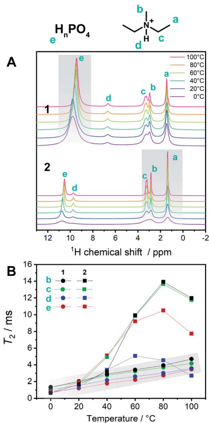
Fig. 5 (A) 1 H SSNMR spectra of 1 and 2 from 0 to 100 °C including the assignments of protons. Narrowing of phosphates peaks in 1 upon heating is highlighted. (B) T_2 of 1 H SSNMR signals of 1 (circles, gray highlight) and 2 (squares) at each temperature.
