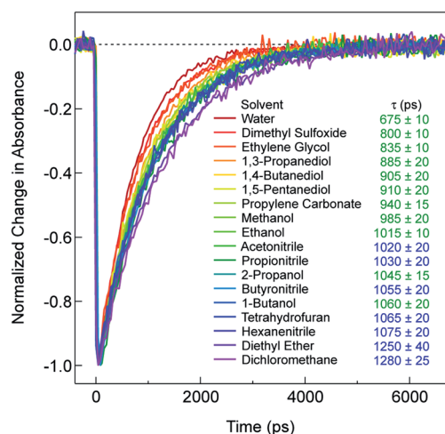
Fig. 1 Time constants for ground-state recovery of [\text{Fe}(\text{bpy})_3]^{2+} in different solvents following ^1A_1 \rightarrow ^1\text{MLCT} excitation at 550 nm. The lifetimes are color-coded based on the counterion used for [\text{Fe}(\text{bpy})_3]^{2+} in a given solvent ( \text{Br}^- (green) and \text{BARF}_4^- (blue)).
