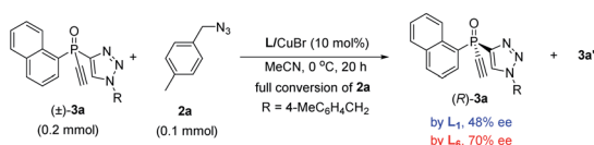
Scheme 2 Reaction profiles.
