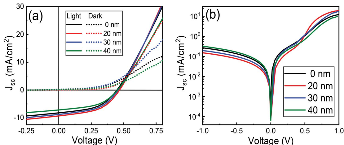
Fig. 15 (a) I - V characteristics under light and dark of 10% cobalt doped ZnO/CuO/MoO 3 heterojunction solar cells with a different thickness of the MoO 3 buffer layer. (b) Semi-log plot of dark I/V for one diode model fit.
