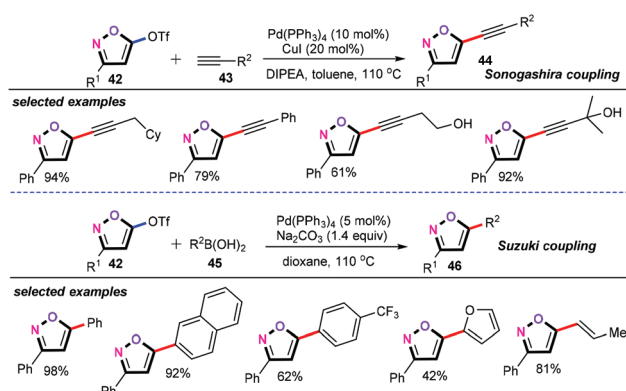
Scheme 21 Palladium-catalyzed coupling of 5-(pseudo)halogenated isoxazoles.
