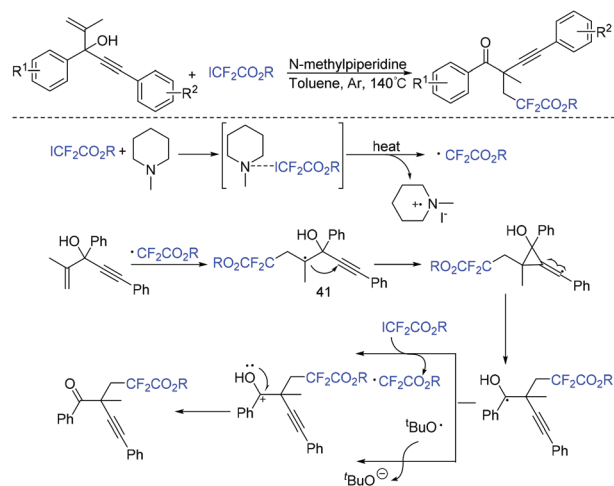
Scheme 20 The base-promoted difluoroalkylation reaction of 1,4-enynes with \text{ICF}_2\text{CO}_2\text{Et} .
