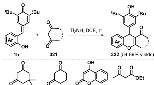
Scheme 71 [4 + 2] annulation of p -QMs with ketones.
