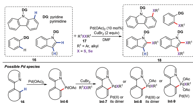
Scheme 6 Palladium-catalyzed intermolecular C–H chalcogenation of arenes and heteroarenes.
