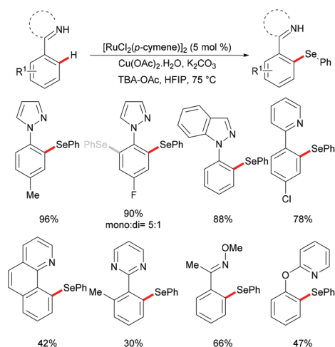
Scheme 28 Ruthenium-catalysed C–H selenylations of arenes with selenyl chlorides.
