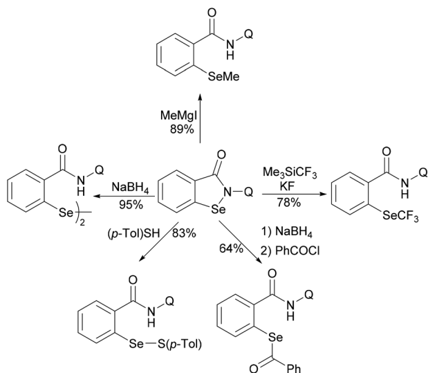
Scheme 74 Further transformation of benzoisoseleazolone.
