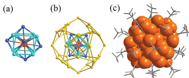
Fig. 16 (a) The \text{Ag}@ \text{Ag}_{14} core; (b) the structure of the \text{Ag}@ \text{Ag}_{14}@ \text{Ag}_{36} shell; and (c) overall structure of \text{Ag}_{51}(\text{tBuC}\equiv\text{C})_{32} . Adapted with permission from ref. 36. Copyright 2018, Royal Society of Chemistry.
