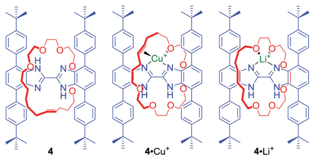
Fig. 2 Loeb's rotaxane 4 and its complexes with \text{Cu}^+ and \text{Li}^+ .
