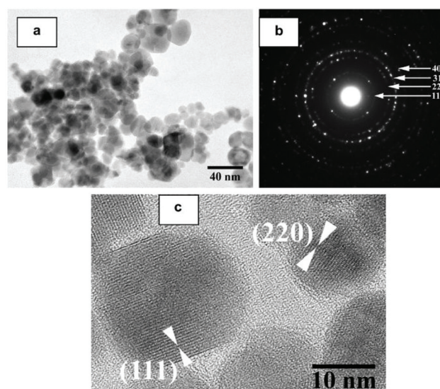
Fig. 8 (a) Bright field TEM micrograph, (b) selected area diffraction and (c) HRTEM image of hydrothermally prepared nanocrystalline \text{Mn}_{0.8}\text{Zn}_{0.2}\text{Fe}_2\text{O}_4 . Reprinted with permission from Nalbandian et al. 194
