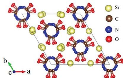
Fig. 10 The crystal structure of \beta\text{-Sr}_3(\text{C}_3\text{N}_3\text{O}_3)_2 .
