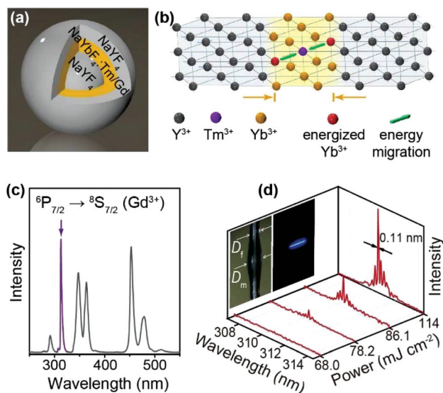
Fig. 8 Yb-Based UCNPs for upconversion lasing. (a) Schematic design of sandwich-structured \beta\text{-NaYF}_4\text{@NaYbF}_4\text{:Tm}^{3+}/\text{Gd}^{3+} (1/30 mol% \text{@NaYF}_4 UCNPs. (b) Schematic illustration of energy transfer from \text{Yb}^{3+} to \text{Tm}^{3+} in the Yb-sublattice. (c) Emission spectrum of the \beta\text{-NaYF}_4\text{@NaYbF}_4\text{:Tm}^{3+}/\text{Gd}^{3+} (1/30 mol% \text{@NaYF}_4 UCNPs under 980 nm excitation. (d) Lasing spectra of the micro-resonator containing the \beta\text{-NaYF}_4\text{@NaYbF}_4\text{:Tm}^{3+}/\text{Gd}^{3+} (1/30 mol% \text{@NaYF}_4 UCNPs as gain media under excitation of 980 nm at different power densities. Insets: Photographs of the micro-resonator without and with optical excitation. D_f and D_m denote diameters of the support fibre and microcavity, respectively. Reprinted with permission from ref. 28. Copyright 2016 Springer Nature.
