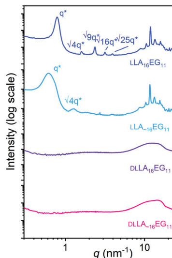
Fig. 2 Wide-angle X-ray scattering (WAXS) data for \text{L}(\text{LA}_{16}\text{EG}_{11}) (blue), \text{L}(\text{LA}_{\sim 16}\text{EG}_{11}) (light blue), \text{DL}(\text{LA}_{16}\text{EG}_{11}) (purple), \text{DL}(\text{LA}_{\sim 16}\text{EG}_{11}) (pink). The data is shifted vertically for clarity. Higher order Bragg reflections are indicated if present.
