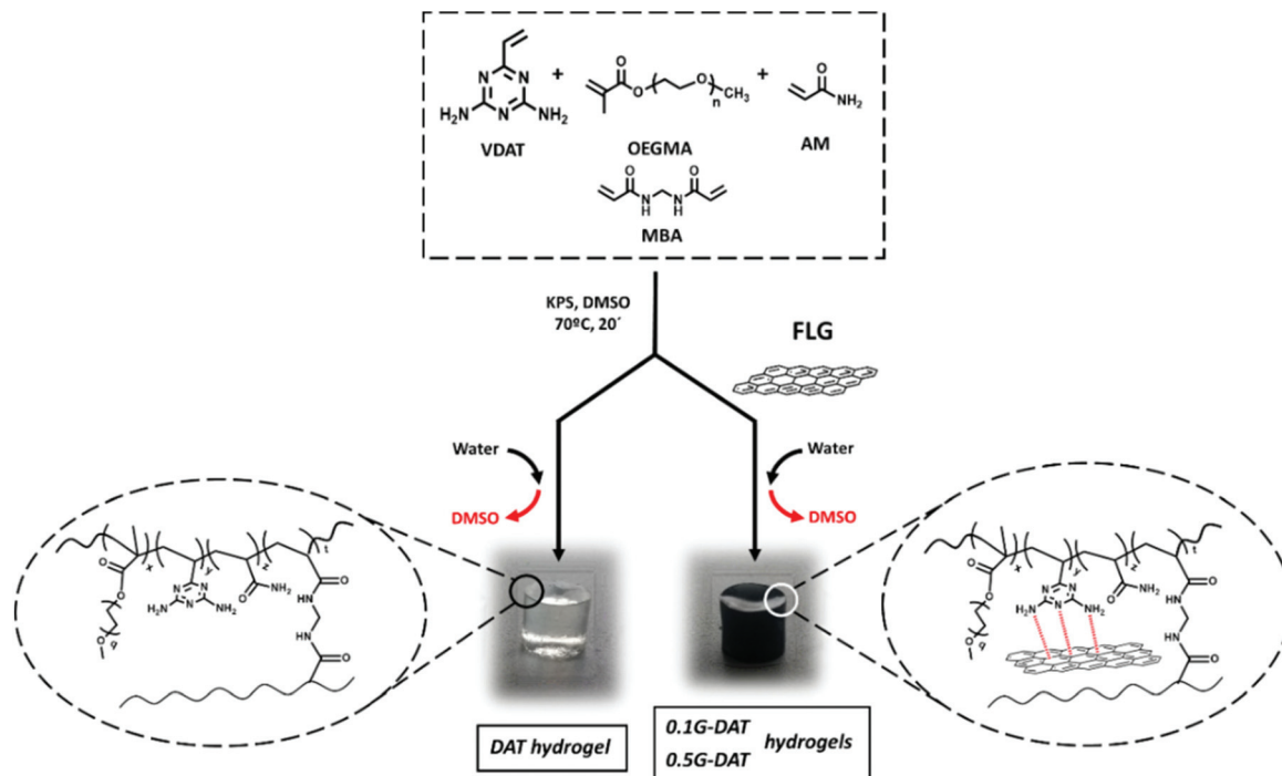
Fig. 1 Synthesis of DAT and G-DAT hydrogels.
