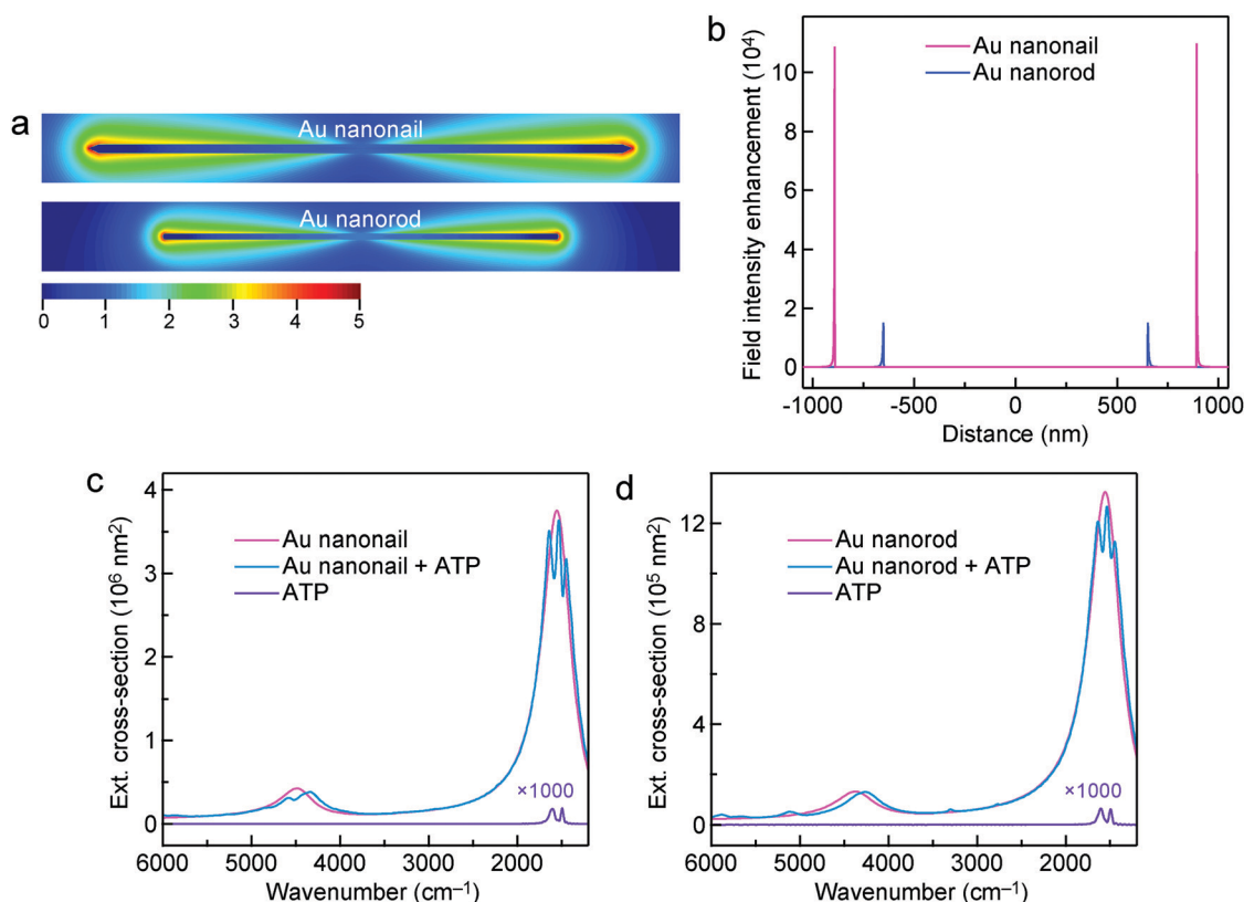
Fig. 6 FDTD simulations. (a) Electric field intensity enhancement ( |E/E_0|^2 ) contours of the Au nanonail and nanorod under the longitudinal excitation at 1555\text{ cm}^{-1} . The lengths/diameters of the Au nanonail and nanorod are 1784 nm/32 nm and 1304 nm/18 nm, respectively. The contours are drawn at the logarithmic scale. (b) Electric field intensity enhancement ( |E/E_0|^2 ) profiles along the longitudinal direction of the Au nanonail and nanorod. The origin is at the center of the Au nanocrystals. (c) Extinction cross-sections of the Au nanonail, the Au nanonail encapsulated with ATP molecules, and the sole shell composed of ATP molecules. (d) Extinction cross-sections of the Au nanorod, the Au nanorod encapsulated with ATP molecules, and the sole shell composed of ATP molecules.
