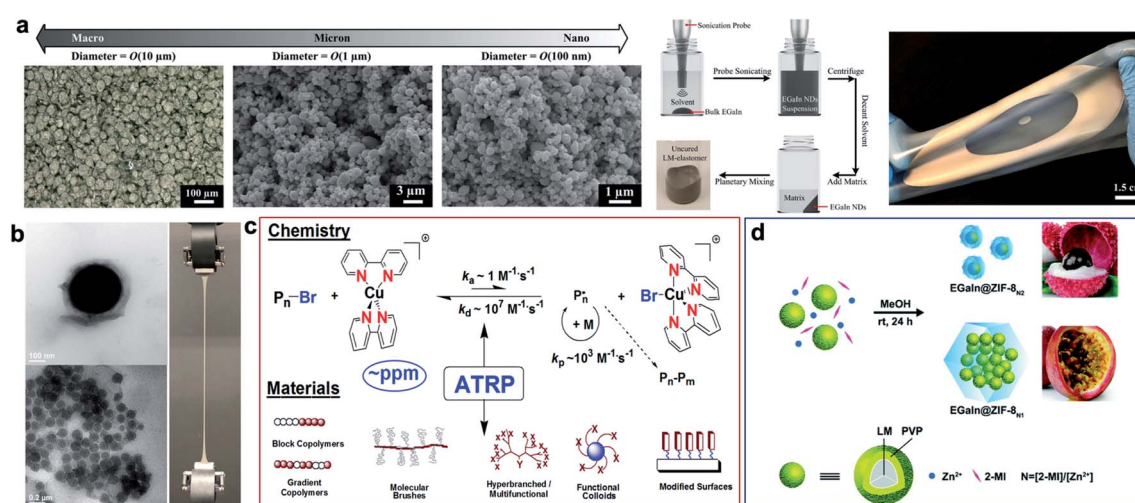
Fig. 2 Synthesis of LM-polymer composites. (a) Left: microscopic images of EGaIn micro/nanodroplets with diameter of O(10 \mu\text{m}) , O(1 \mu\text{m}) , and O(100 \text{ nm}) . The far left image presents the top view of a composite with an elastomer matrix and O(10 \mu\text{m}) droplets made by shear mixing bulk EGaIn with elastomer. Center: schematic shows the preparation of LM-nanocomposites. Right: image of stretched LM-elastomer nanocomposite (silver; annular shape) on a silicone elastomer carrier film (semitransparent). Reproduced with permission, 12 copyright 2019, Wiley-VCH. (b) LM-nanocomposites prepared by surface-initiated atom transfer radical polymerization. Reproduced with permission, 41 copyright 2019, Nature Publishing Group. (c) Schematic illustration of atom transfer radical polymerization (ATRP) and materials made by this technique. (d) Schematic illustration of the synthesis of "litchi"- and "passion fruit"-like EGaIn@ZIF-8 NPs. Pre-synthesized EGaIn@PVP nanodroplets are mixed with 2-methylimidazole (2-MI) and \text{Zn}^{2+} at different L/M ratios ( N = 2 and 1). Reproduced with permission, 49 copyright 2020, Royal Society of Chemistry.
