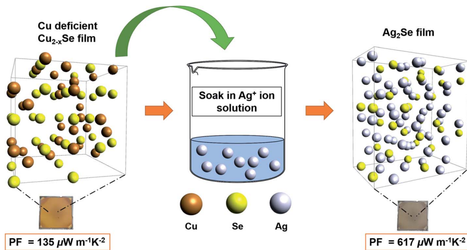
Fig. 1 Schematic describing the process in which a Cu-deficient \text{Cu}_{2-x}\text{Se} thin film transforms into a \text{Ag}_2\text{Se} thin film by fully immersing the \text{Cu}_{2-x}\text{Se} thin film into a \text{Ag}^+ -rich solution for different amounts of time followed by annealing. \text{Ag}^+ concentration gradient is established between the soaking solution and the thin film drives the \text{Ag}^+ ions to diffuse into the \text{Cu}_{2-x}\text{Se} crystal lattice and replace the \text{Cu}^+ ions. Electrically, this process results in a switching of majority carrier type from p-type ( \text{Cu}_{2-x}\text{Se} ) to n-type ( \text{Ag}_2\text{Se} ) and an increase in the average PF from 135 \mu\text{W m}^{-1} \text{K}^{-2} to 617 \mu\text{W m}^{-1} \text{K}^{-2} . The photographs show the \text{Cu}_{2-x}\text{Se} film (before soak) and the \text{Ag}_2\text{Se} film (after soak) on glass substrates.
