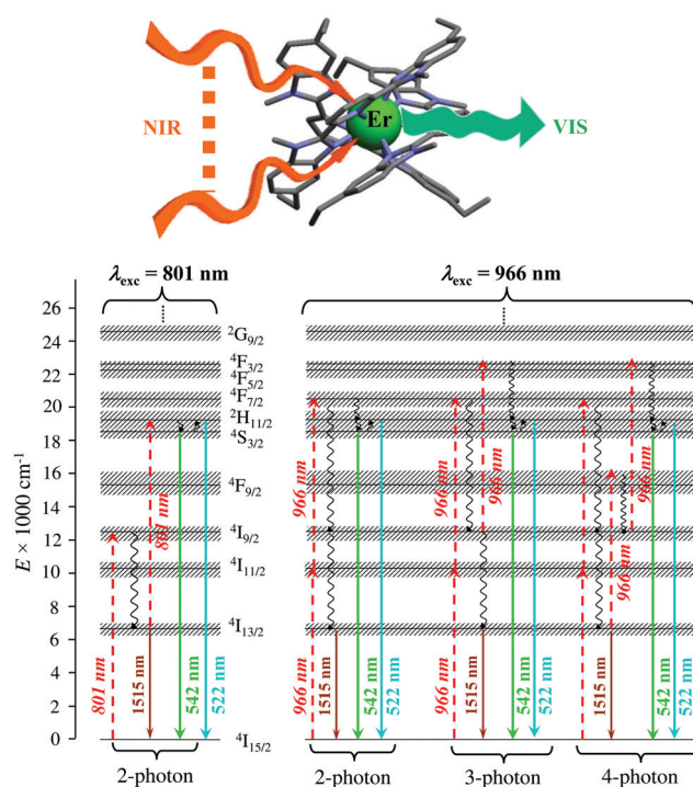
Fig. 20 Molecular structure and energy diagram summarizing the mechanisms of the Er-centred upconversion processes operating in [\text{Er}(\text{L5})_3]^{3+} upon excitation of the \text{Er}({}^4\text{I}_{9/2} \leftarrow {}^4\text{I}_{15/2}) transition at 801 nm (left) or of the \text{Er}({}^4\text{I}_{11/2} \leftarrow {}^4\text{I}_{15/2}) transition at 966 nm (right). Excitation (dashed upward arrows), non-radiative multiphonon relaxation (downward curled arrows), thermal equilibria (upward curled arrows) and radiative emission processes (straight downward arrows). 65,80
