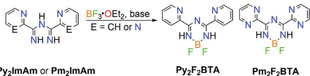
Scheme 6 General synthetic route used for the synthesis of 2,2-difluoro-4,6-bis(2-pyridyl)-1,3,5-dihydro-1,3,5,2-triazaborinine ( Py 2 F 2 BTA ) and 2,2-difluoro-4,6-bis(2-pyrimidinyl)-1,3,5-dihydro-1,3,5,2-triazaborinine ( Pm 2 F 2 BTA ). Reagents and conditions: ( Py 2 F 2 BTA ) triethylamine (Et 3 N), tetrahydrofuran (THF), 60 °C; ( Pm 2 F 2 BTA ) Et 3 N, dichloromethane (DCM).
