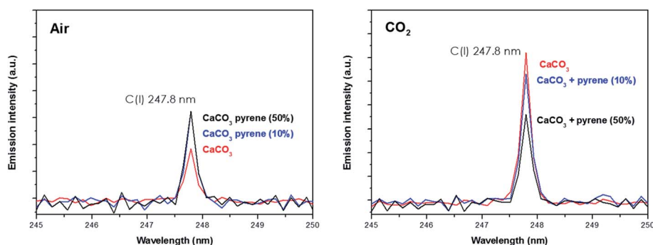
Fig. 4 Emission intensity of the atomic carbon signal from both the pure \text{CaCO}_3 matrix and that doped with 10% pyrene in both air and the \text{CO}_2 atmosphere.
