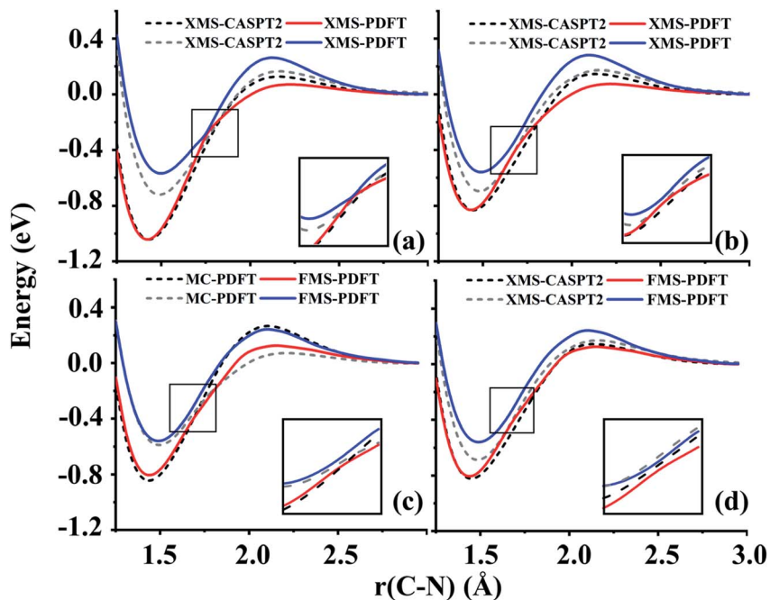
Fig. 3 (a) and (b) Comparison of XMS-PDFT with XMS-CASPT2 for the two lowest potential energy curves along the CN bond dissociation of HNCO with the \tau(\text{HNCO}) torsion angle at 175° and 150° respectively. (c) and (d) Comparison of FMS-PDFT with MC-PDFT and XMS-CASPT2 for the two lowest potential energy curves along the CN bond dissociation with the \tau(\text{HNCO}) torsion angle at 150°. The curves from 2.0 to 2.5 Å are calculated with numerically optimized VMS-PDFT instead of FMS-PDFT.
