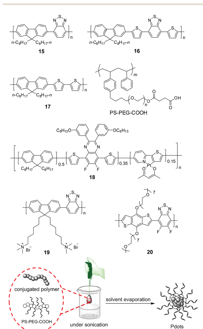
Fig. 6 Chemical structures of polymers 15–20 and preparation of polymer dots (Pd dots) by the nano-precipitation method for photocatalytic \text{H}_2 production. The scheme is adapted with permission from ref. 82, Copyright 2016 Wiley-VCH.
