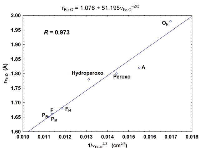
Fig. 9 Correlation between the calculated Fe a3 –O bond lengths ( r Fe–O , Å) and the corresponding Fe a3 –O stretch frequencies ( 1/\nu_{\text{Fe–O}}^{2/3} , based on Badger's rule) for the eight DNC state structures studied. 59 Reprint with permission from Fig. 7 of ref. 59, copyright© 2019 American Chemical Society.
