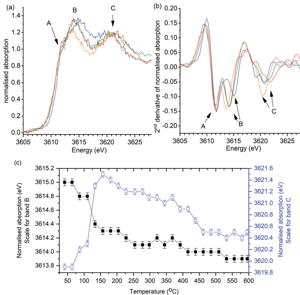
Fig. 3 Control operando potassium K-edge XANES of \text{K}/\alpha\text{-Al}_2\text{O}_3 during heating to 600 °C in the absence of soot. Heating rate of 2 °C \text{min}^{-1} (a) Selection of normalised XANES data showing key changes in catalyst structure during reaction. (b) 2nd derivative of data processed XANES spectra shown in (a). XANES scan at: 40 °C (blue), 160 °C (red), 300 °C (green) and 600 °C (orange). Fig. 6c shows recorded energy of features B (1s \rightarrow 4d) and C (multiple scattering feature) at all recorded temperatures. Error of \pm 0.1 eV determined as confidence in measuring peak maximum.
