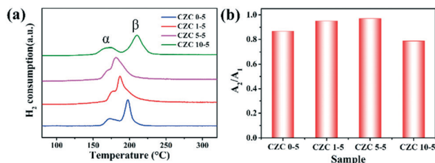
Fig. 6 (a) \text{H}_2 -TPR profiles and (b) cumulative \text{H}_2 uptake of the different CZC samples.
