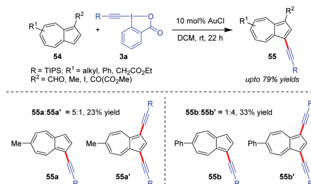
Scheme 11 Direct alkylnation of azulenes.
