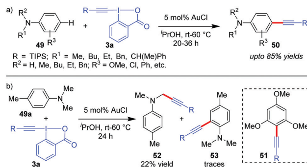
Scheme 10 para -Selective direct alkylnation of anilines.
