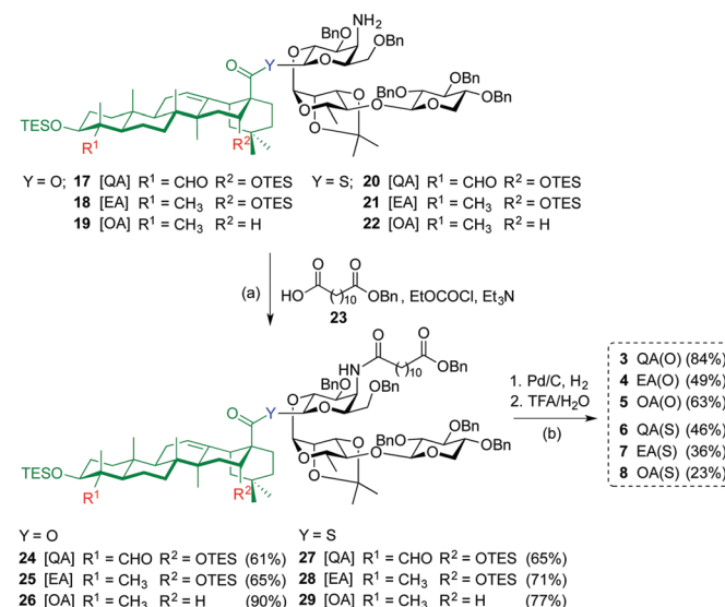
Scheme 2 Reagent and conditions: (a) \text{EtOCOC}(\text{O})\text{CH}_2(\text{CH}_2)_{10}\text{OBn} , \text{Et}_3\text{N} , THF, 0 °C to r.t., 4 h, 61% (for 24), 65% (for 25), 90% (for 26); 65% (for 27), 71% (for 28), and 77% (for 29); (b) 1: Pd/C, \text{H}_2 (1 atm), \text{EtOH}/\text{THF} 1 : 1, r.t., 16 h (for 24–26); 20 min (for 27–29); 2: TFA/ \text{H}_2\text{O} 3 : 1, 0 °C, 1 h, 84% (for 3), 49% (for 4), 63% (for 5); 46% (for 6), 36% (for 7), and 23% (for 8).
