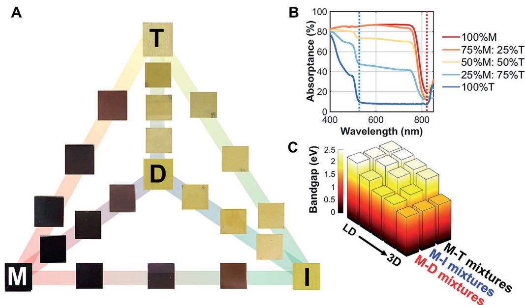
Fig. 2 Optical properties of the 3D/low dimensional perovskites studied here. (A) Thin films of methylammonium lead iodide (M) mixed with dimethylammonium lead iodide (D), iso-propylammonium lead iodide (I), and t -butylammonium lead iodide (T) with set ratios: 100% : 0%, 75% : 25%, 50% : 50%, 25% : 75%, and 0% : 100%. The 100% M, D, I, and T films are indicated with the corresponding letters on the films. (B) Absorption of the M–T series, where two absorption onsets are shown at 525 and 825 nm. (C) The direct bandgap estimated by Tauc plots for the M–D, M–I, and M–T series at the 525 nm onset; a secondary phase bandgap estimation resulting from the 825 nm onset is shown in ESI Fig. S7.†
