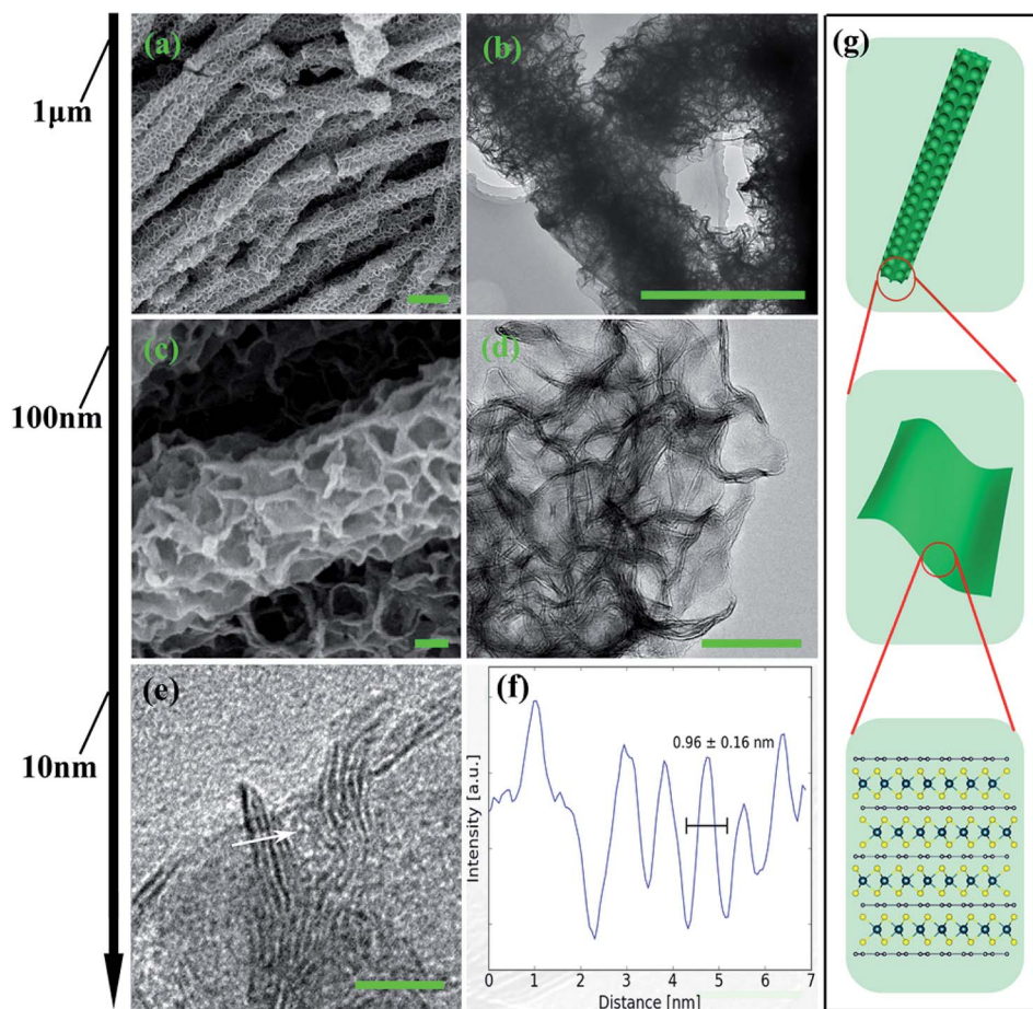
Fig. 5 Structural organisation of MoS 2 /NC-PNR on several length scales: (a, c) SEM images (scale bar 1 μm), (b, d) TEM images (scale bar 100 nm), (e) HR-TEM images (scale bar 10 nm), (f) line scan of the white arrow in (e) and (g) schematic illustration of the hierarchical structure.
