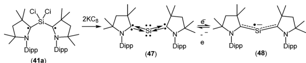
Fig. 13 cAAC-stabilized siladibene and in situ generation of ( ^{\text{Me}2}\text{cAAC} ) 2 Si 2− .
