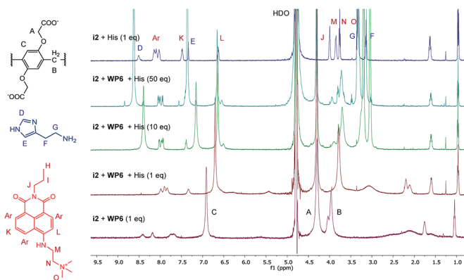
Fig. 8 ^1\text{H} -NMR spectra (500 MHz, \text{D}_2\text{O} , 0.5 mM) of the indicator displacement of \text{i2} \cdot \text{WP6} mixture in the presence of histamine in different concentrations. The uppermost spectrum is a mixture of \text{i2} and histamine.
