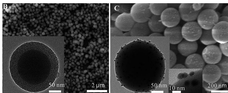
Fig. 13 (A) Schematic illustration of the procedure for the preparation of mSiO 2 @NH 2 @Ag. (B) SEM image of mSiO 2 microspheres. (C) SEM image of mSiO 2 @NH 2 @Ag. The insets show the low-magnification and high-magnification TEM images of mSiO 2 @NH 2 @Ag 41 (adapted with permission from Royal Society of Chemistry, 2015).
