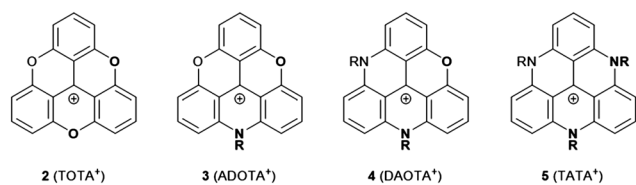
Fig. 3 Schematic representation of O- and/or N-bridged trianguleniunium cations 2–5 (R denotes an alkyl or aryl residue, the counterions are omitted for clarity).
