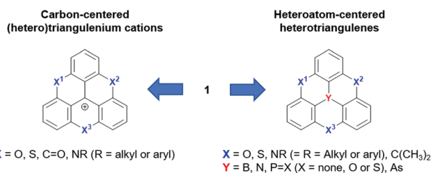
Fig. 2 Schematic representation of the carbon-centered trianguleniunium and heteroatom-centered triangulene derivatives deduced from the parent compound 1 .
