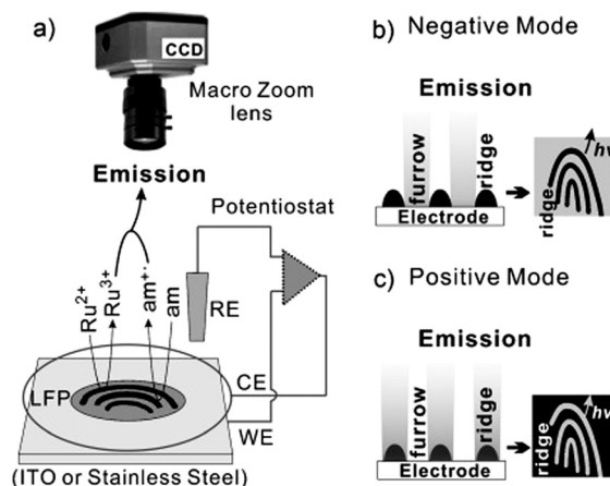
Fig. 15 (a) The ECL imaging system: \text{Ru}^{2+} and \text{am} represent the ECL generating luminophore and the amine co reactant, respectively. (b and c) The imaging strategy for visualizing LFPs in the negative (b) and positive (c) mode. 109 Reprinted with permission from ref. 109. Copyright 2012 Wiley-VCH Verlag GmbH & Co. KGaA, Weinheim.
