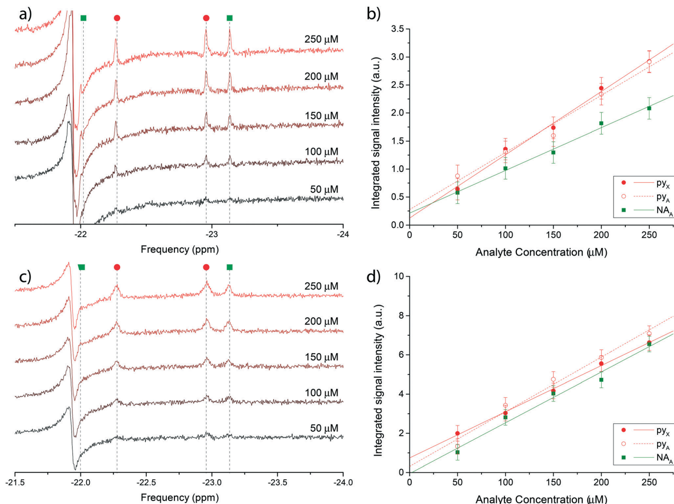
Fig. 4 a) Single scan 1 H @500 MHz NMR spectra of a nicotinamide and pyridine concentration series ranging from 50 μM to 250 μM, performed in bulk on a Bruker Micro-5 NMR probe. c) 128-averaged spectra of the concentration series recorded on the micro-NMR setup. Peak assignment in (a) and (c) follows the colour scheme reported in Fig. 3. (b and d) Corresponding signal integrals of di-hydride peaks in plots (a) and (c) as a function of nominal nicotinamide and pyridine concentrations. The X hydride for nicotinamide was not quantified due to the overlap with a constant antiphase signal in the same region. The mass sensitivity range corresponding to the concentration range covered by the experiments is 15–75 pmol.
