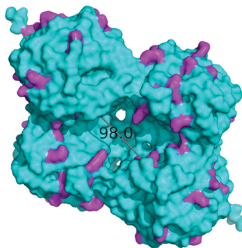
Fig. 4 MeHNL tetramer surface representation (longest extension: 98.0 Å). 60 Surface lysine residues are highlighted in magenta. X-ray structure 1DWP36 was obtained from the PDB38 and the image was created using the PyMOL Molecular Graphics System. 37
