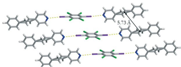
Fig. 1 X-ray structure of form I illustrating the I...N halogen bonds as well as the offset homogeneous \pi - \pi stacking arrangement of C 6 I 2 Cl 4 . The I...N halogen bonds are shown with yellow dashed lines.
