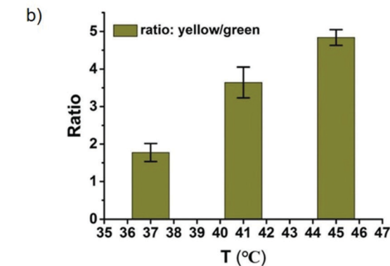
Fig. 63 Relationship between lysosomal pH changes and heat stroke in HeLa cells. (a) Ratiometric fluorescence images of the 42 -stained cells under heat shock at 37^\circ\text{C} , 41^\circ\text{C} , and 45^\circ\text{C} (left to right) respectively for 20 min and then continued culture for another 20 min at 37^\circ\text{C} . Excitation wavelength for probe 42 : 488 nm; emission collection, channel 1 (green, channel 1): 500–550 nm; channel 2 (yellow, channel 2): 570–620 nm. Scale bar is 10 \mu\text{m} . (b) Semiquantitative determination of 42 -stained HeLa cells according to the ratio of average fluorescence intensity of channel 2 (yellow) to channel 1 (green). Error bars represent s.d. Copyright 2018 Royal Society of Chemistry.
